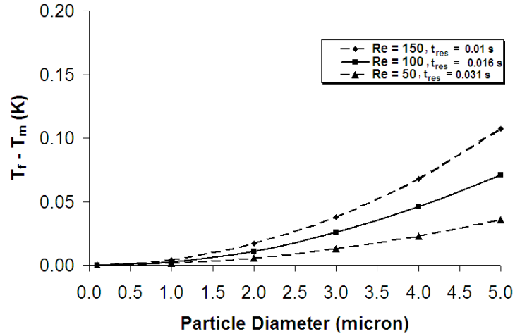
Figure 3-3. T_f - T_m for different particle diameters (base fluid - water)
