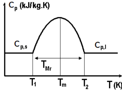
Figure 3-5. Specific heat of EPCM, function of temperature
