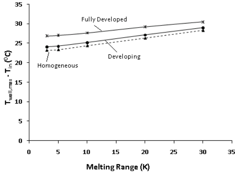
Figure 3-20. T_{wall, max} - T_{in} for all three profiles at different melting ranges
